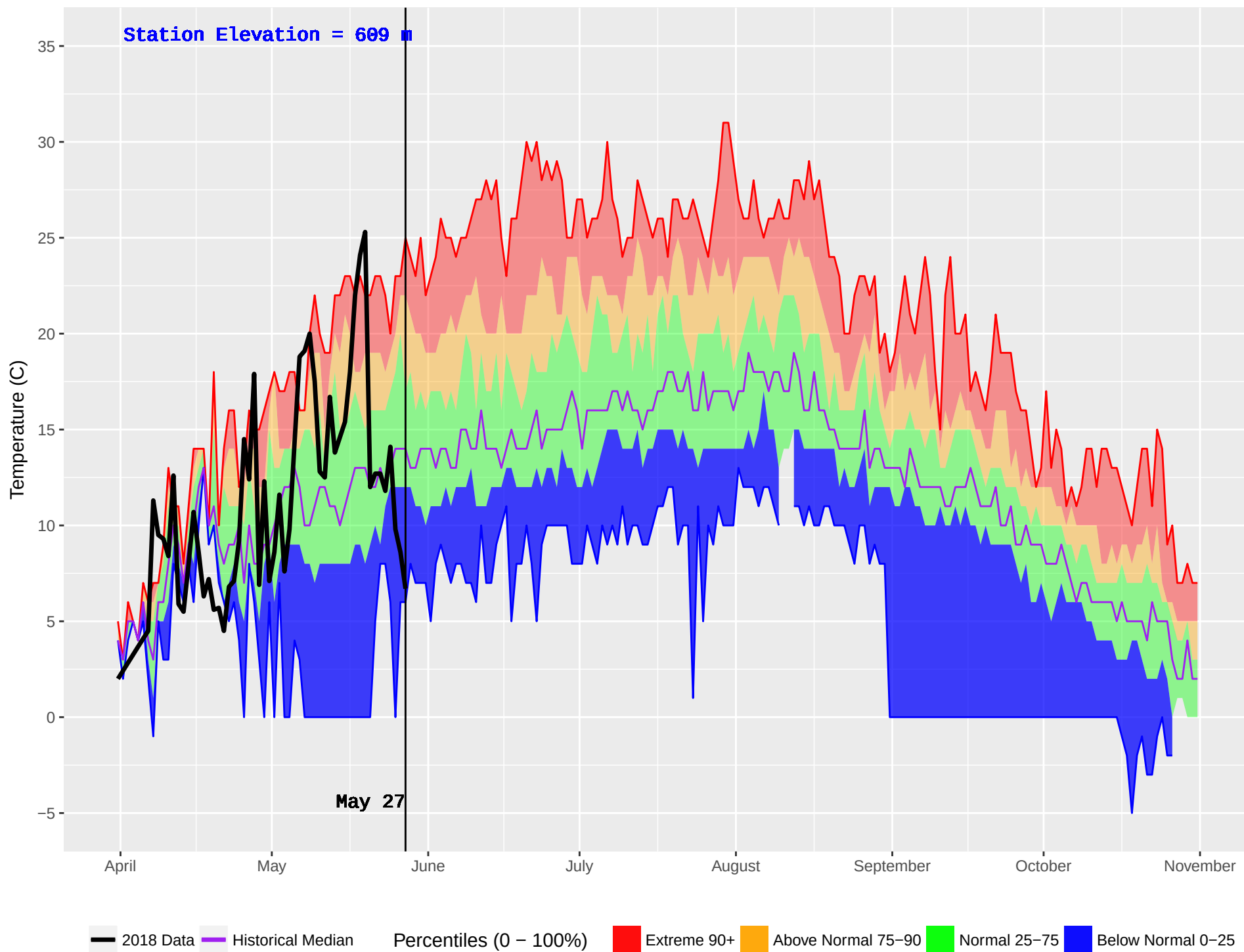
BOB QUINN LAKE (113) : Historical (1984–2016) and Current (2018) Noon Temperature
