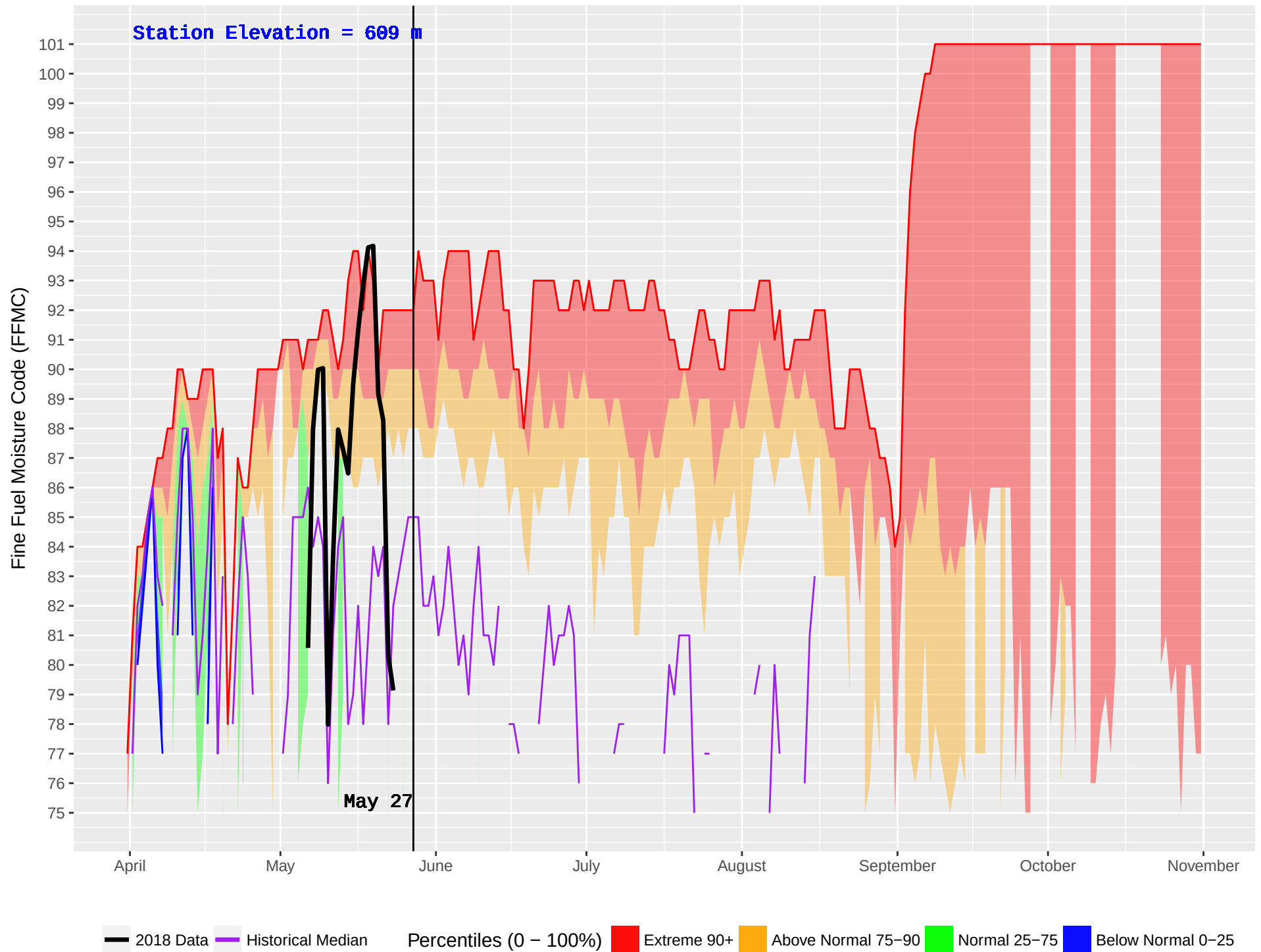
BOB QUINN LAKE (113) : Historical (1984–2016) and Current (2018) Noon Fine Fuel Moisture Code (FFMC)
