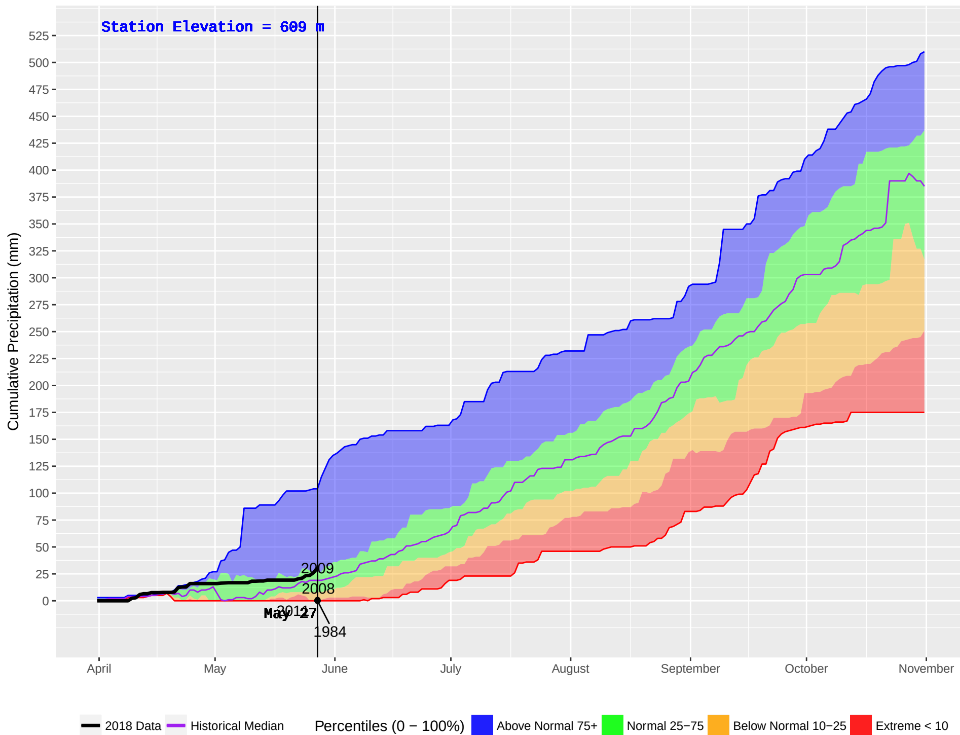
BOB QUINN LAKE (113) : Historical (1984–2016) and Current (2018) Noon Cumulative Precipitation
